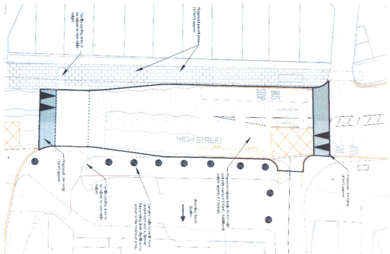
Bromley High Street new stone setts and anti-skid treatment.
